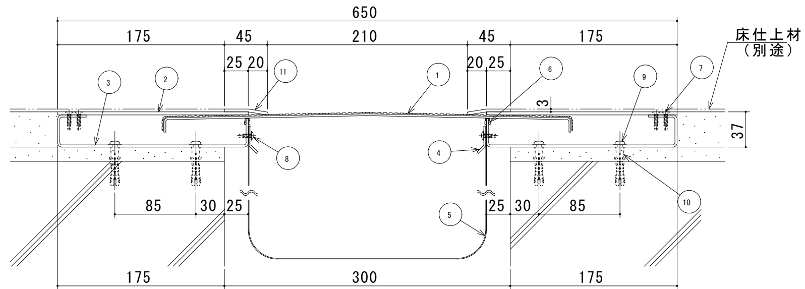
S300-FHM 断面図
