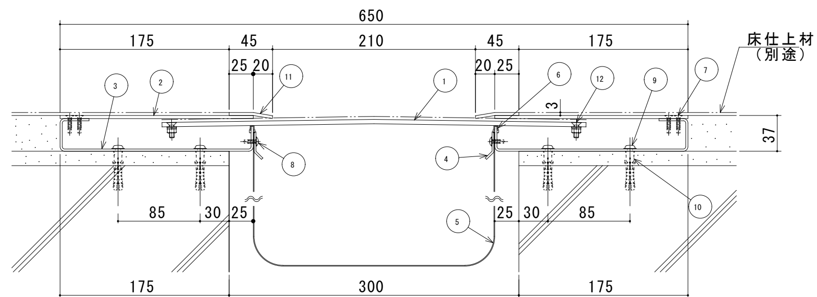
S300-FHMB 断面図
