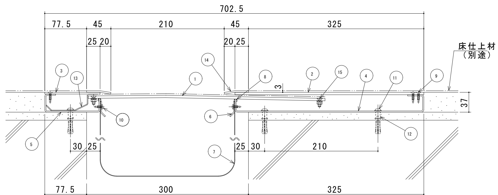
S300-FHMB-AS 断面図
