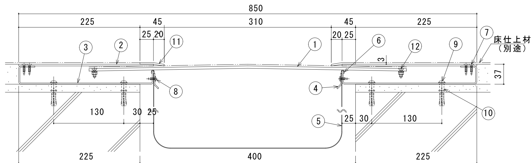
S400-FHMB 断面図
