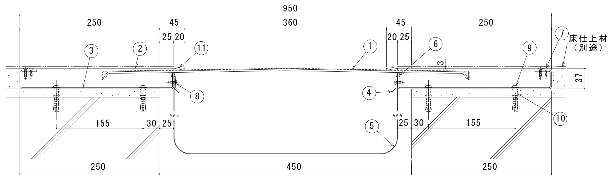
S450-FHM 断面図
