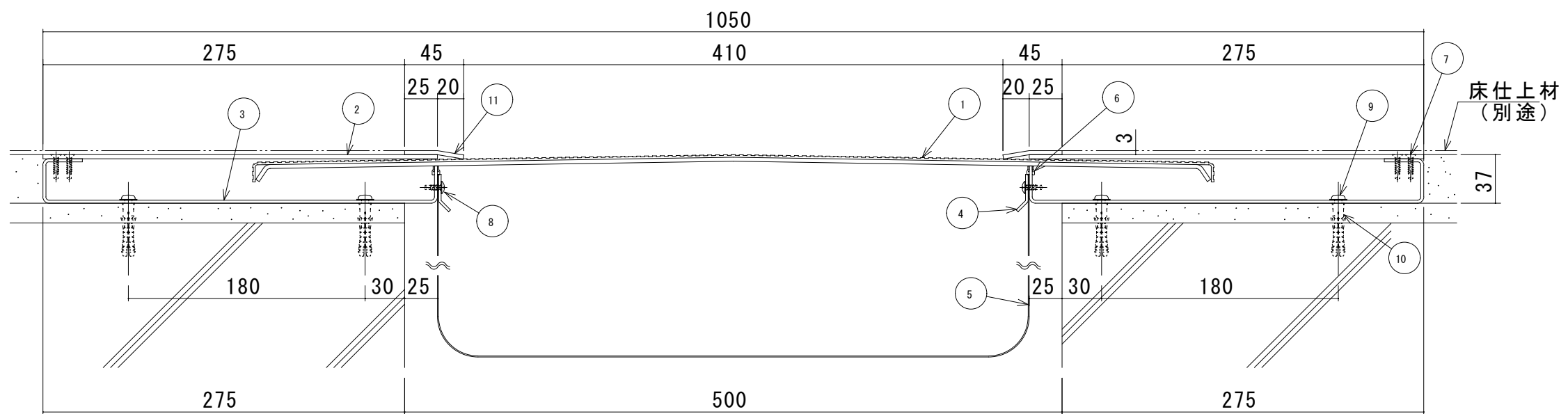
S500-FHM 断面図
