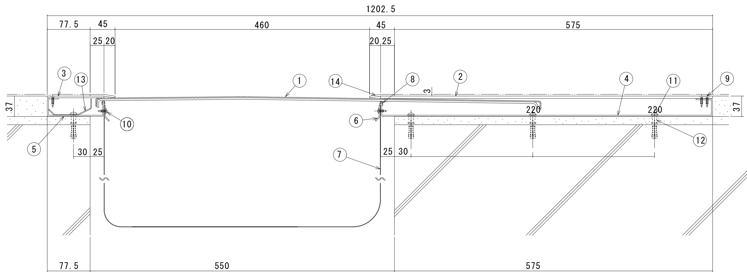
S550-FHM-AS 断面図
