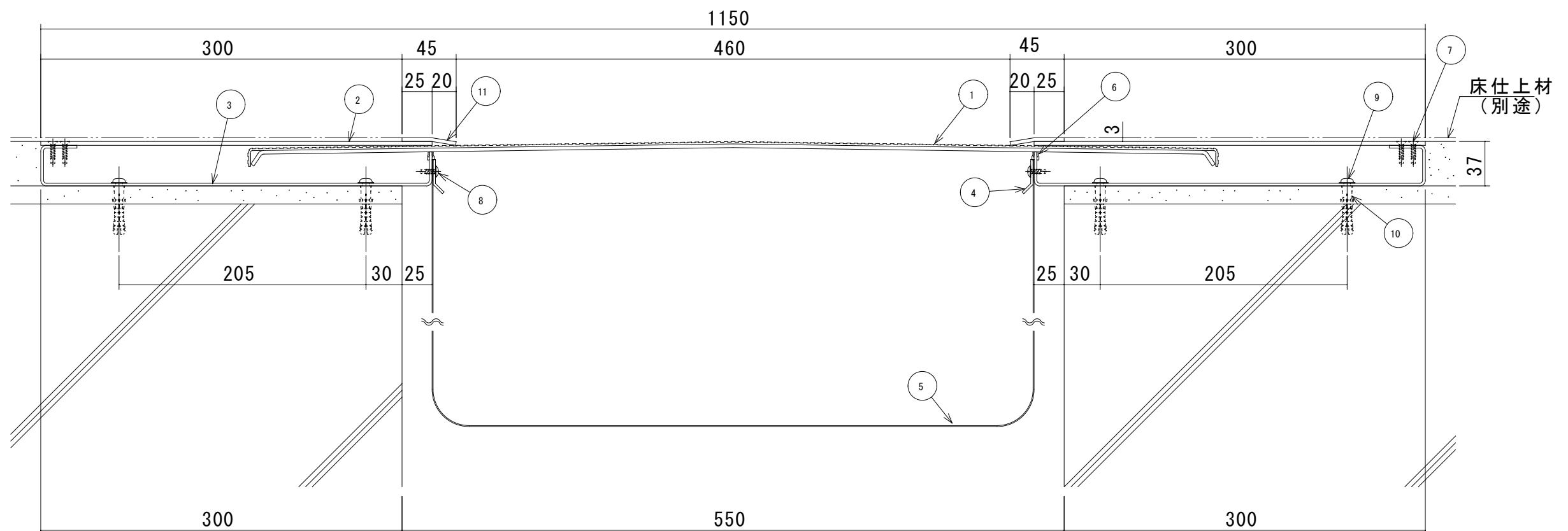
S550-FHM 断面図
