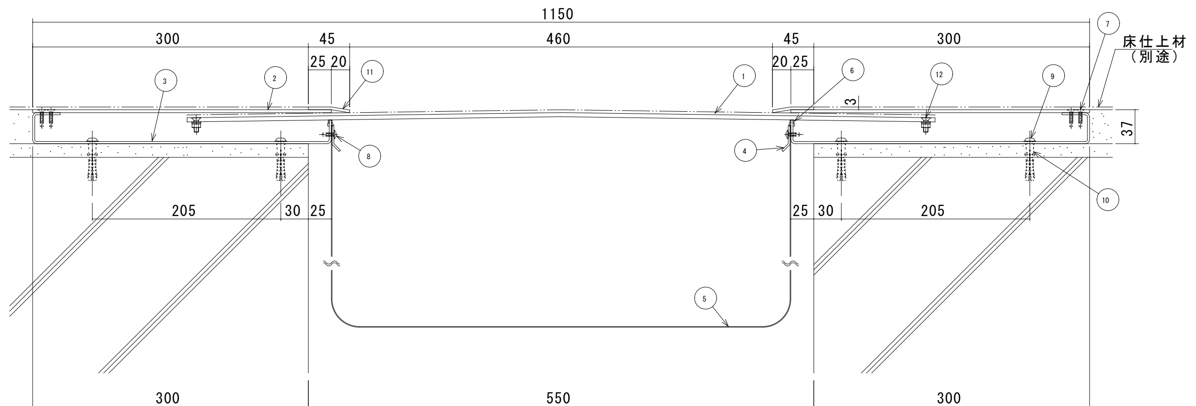
S550-FHMB 断面図
