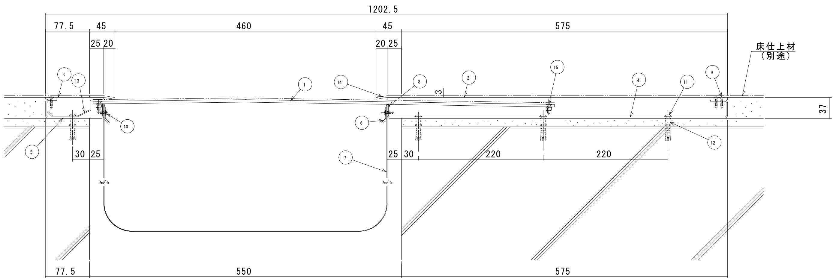
S550-FHMB-AS 断面図
